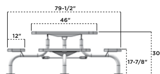
369SM-V Square Span Leg Table, black diamond pattern, black frame
