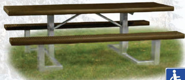
Model WPTS Universal Access Table in 6 ft. or 8 ft. lengths, with V-Type expanded steel or H-Type perforated steel top/seats. (see Page 29)
