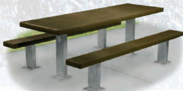
Model APT Multi-Pedestal Tables and APT-X Utility Tables in 6 ft. or 8 ft. lengths, with V-Type expanded steel or H-Type perforated steel top/seats. (see Page 44, 83)
